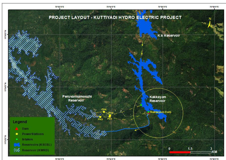
Figure 1.1: Project Layout
