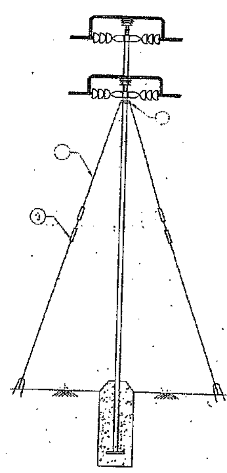
SECTION-B-B
